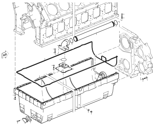
OIL PAN 010.00085
