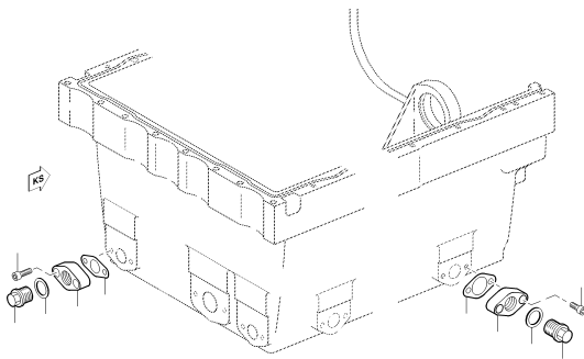
SEAL ELEM. 010.00141
